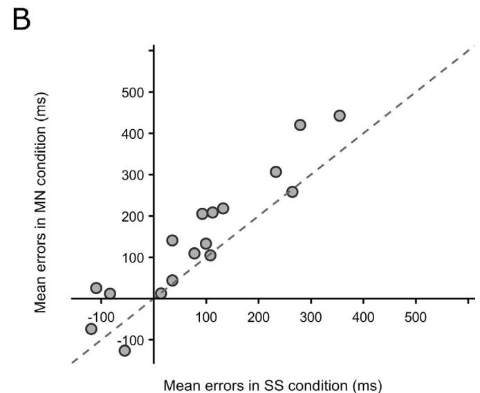
Figure 4. Single observers comparison between mean errors in the key conditions. (A) Single observers mean reproduction errors in the SM condition versus baseline (SS). Each point represent the errors in the two conditions for a given participant. The dashed gray line represents equality between these two measures. (B) single observers mean reproduction errors in the MN condition versus baseline (SS).
